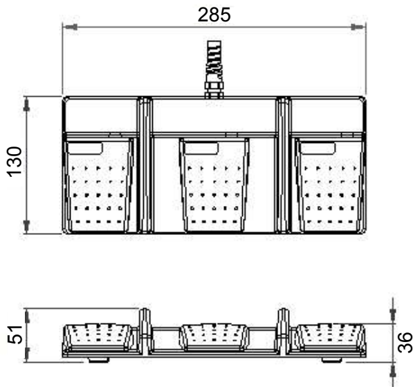
Reference dimensions - 3-pedal model
